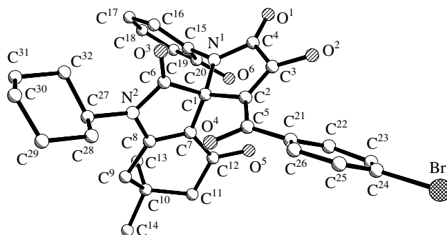
Structure of the molecule of 3'-(4-bromobenzoyl)-1-cyclohexyl-4'-hydroxy-1'-(2-hydroxyphenyl)-6,6-dimethyl-6,7-dihydrospiro[indole-3,2'-pyrrole]-2,4,5'(1 H ,1' H ,5 H )-trione ( IIIi ) according to the X-ray diffraction data.
